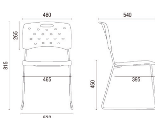
35.008 A VIVA MULTIUSO APILABLE
