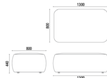
26.222 BLOKZ ASIENTO 2C 1300MM
